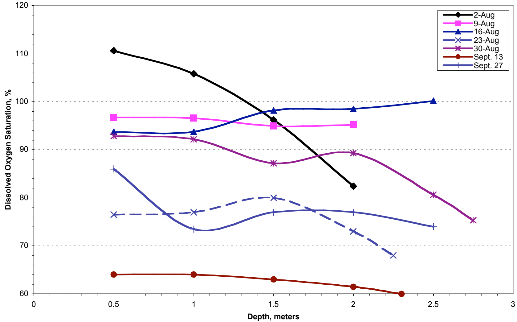
Dissolved Oxygen Saturation versus Depth for Quonnie Pond-Harmonic Cove Buoy Station
